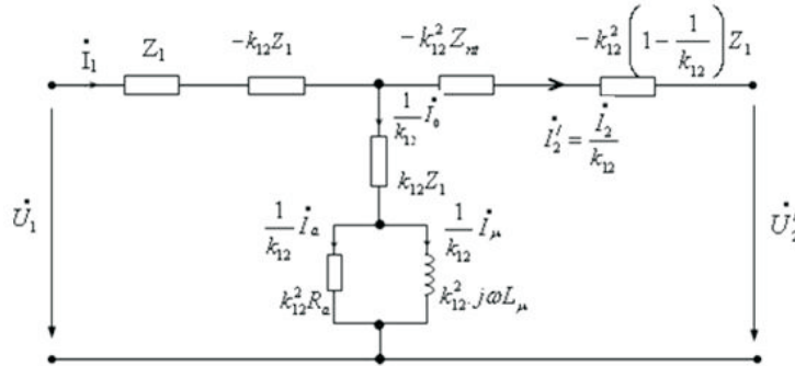
Figure 8. The alternative circuit of the step-up auto-transformer with the no-load current I_0 built from the alternative circuit of the step-down auto-transformer
